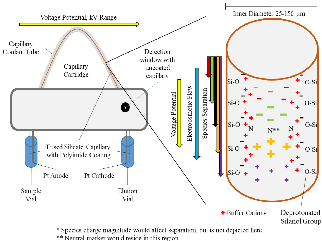
Figure 9. CE cartridge and functional components of the capillary.
